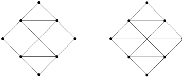
Figure 2.26. Is either of these graphs planar?
