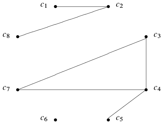
Figure 3.10. The threshold graph G(6) generates the fifth-level clustering \mathbf{C}_5 , which contains one four-element cluster \{c_3, c_4, c_5, c_7\} , one three-element cluster \{c_1, c_2, c_8\} , and a one-element cluster \{c_6\} .
