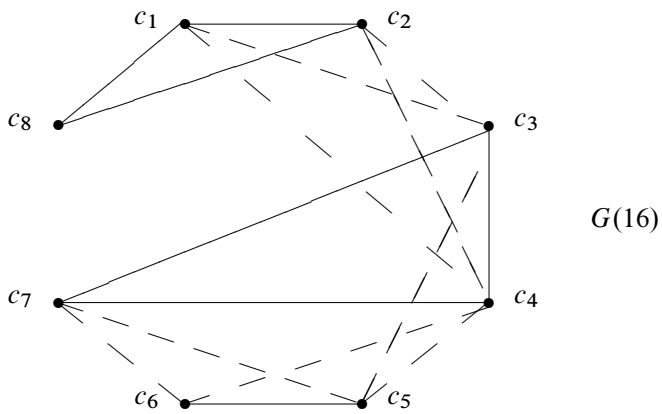
Figure 3.23. Complete linkage: threshold graphs G(15) – G(16) .
