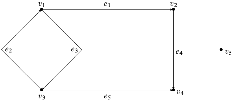
Figure 2.2. Digraph \overline{G} .
