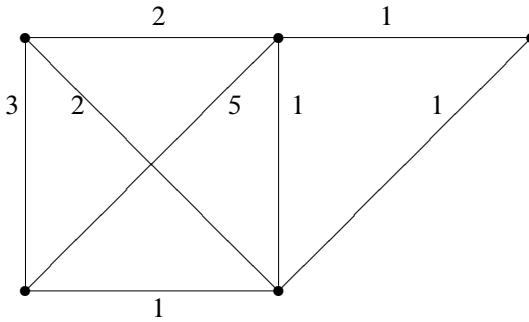
Figure 2.22. Graph G_8 .
