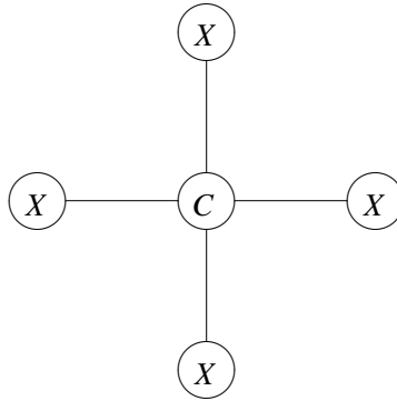
Figure 4.4. Molecules in Problem 4.5.16.
