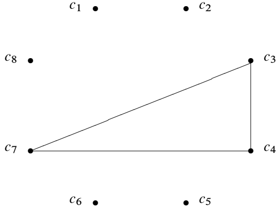
Figure 3.6. The threshold graph G(3) does not generate a new clustering.
