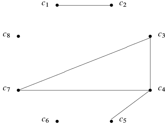
Figure 3.8. The threshold graph G(5) generates the fourth-level clustering \mathbf{C}_4 consisting of one four-element cluster \{c_3, c_4, c_5, c_7\} , one two-element cluster \{c_1, c_2\} , and two one-element clusters \{c_6\} and \{c_8\} .
