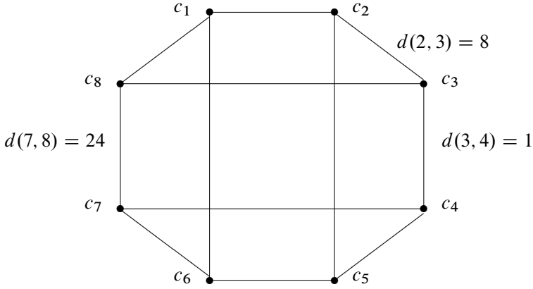
Figure 3.2. The complete threshold graph G(\infty) for the model example; only a few edges and dissimilarities are shown.
