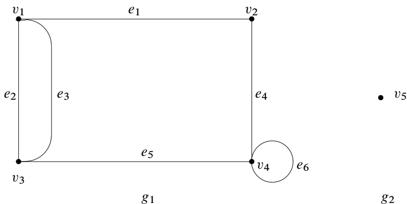
Figure 2.7. Diagrams g_1 and g_2 – see graph G_1 .
