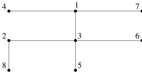
Figure 2.23. This tree has the Prüfer code 133132 – Problem 2.3.6.
