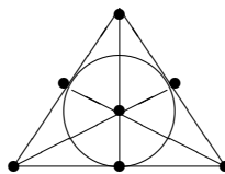
Figure 5.2. The Fano plane.
