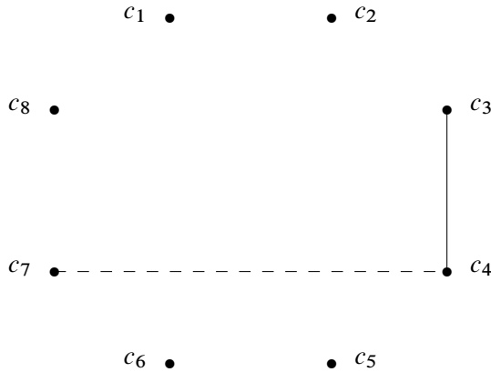
Figure 3.14. The threshold graph G(2) . The edge \{c_4, c_7\} is dashed (cf. Fig. 3.5) for it does not generate the next level complete-link clustering.
